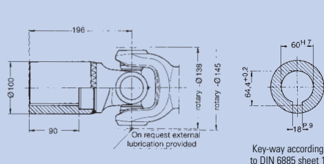
Connecting hub without key-way end number: 0.148.XX2 with key-way end number: 0.148.XX3
