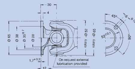
Larger flange end number: 0.105.XX1
