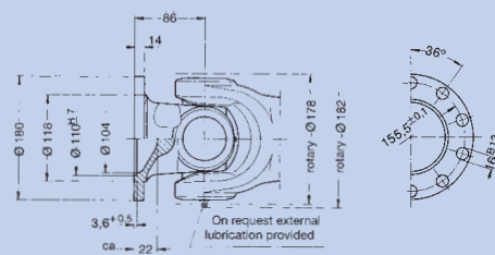
Shorter flange to short type I
