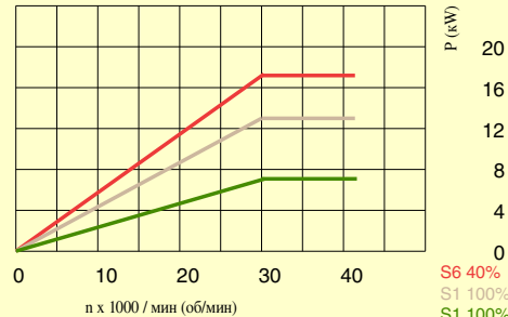
HF 120.2 AI36 - 220V - 55A - 32A
