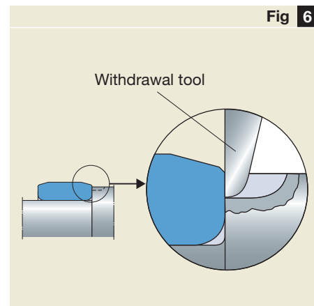
Notches pre-machined in the shaft shoulder that accommodate puller arms eliminate the risk of damaging the inner ring or seating
