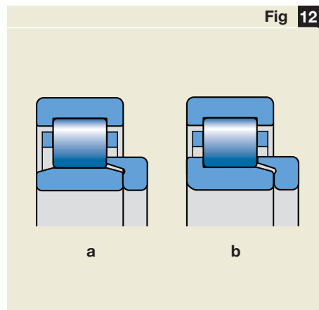
Bearings with an angle ring
